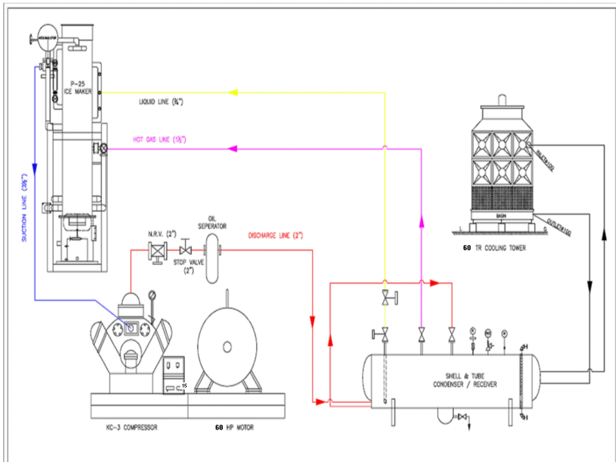
Annexure 1: Process Flow Diagram
