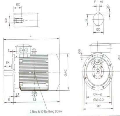
2 Nos. M10 Earthing Screw
