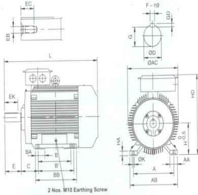
2 Nos. M10 Earthing Screw
